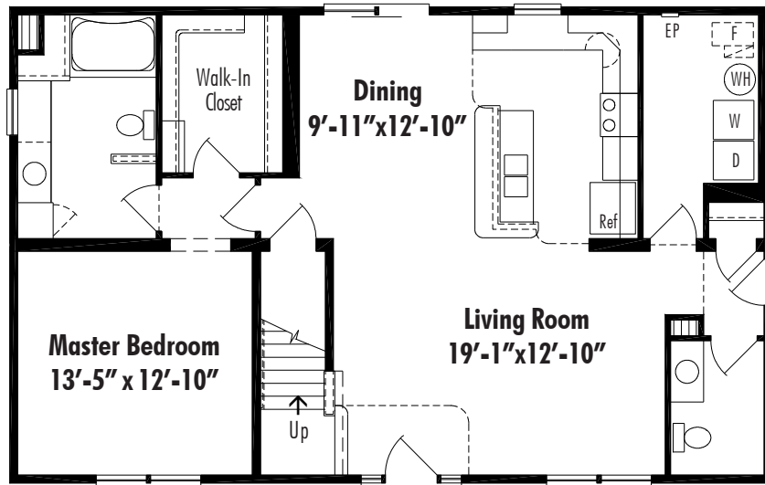
Jefferson I A Crawl Space 27'-4" x 44' 1 / 30 ' 2035 Sq. Ft. Total Living Area
