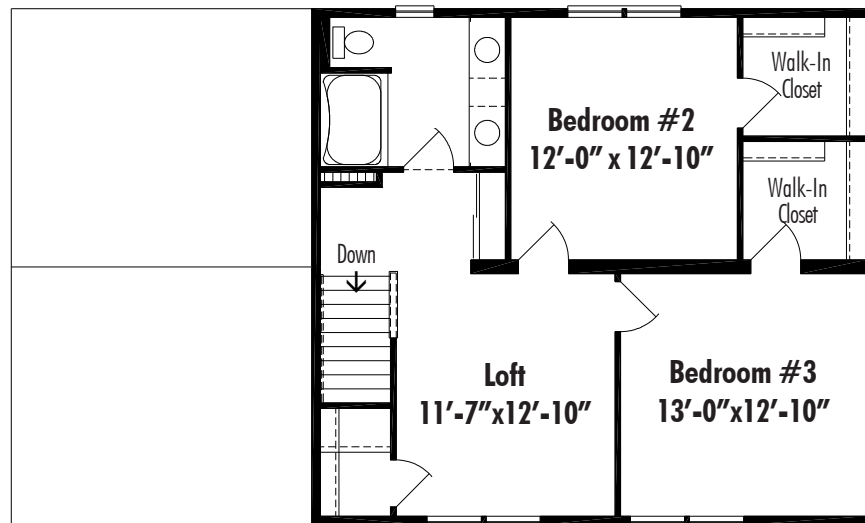
Jefferson I Second Floor 27'-4" x 30'
